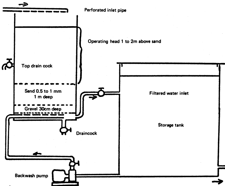
Fig. 21. RAPID GRAVITY SAND FILTERS
