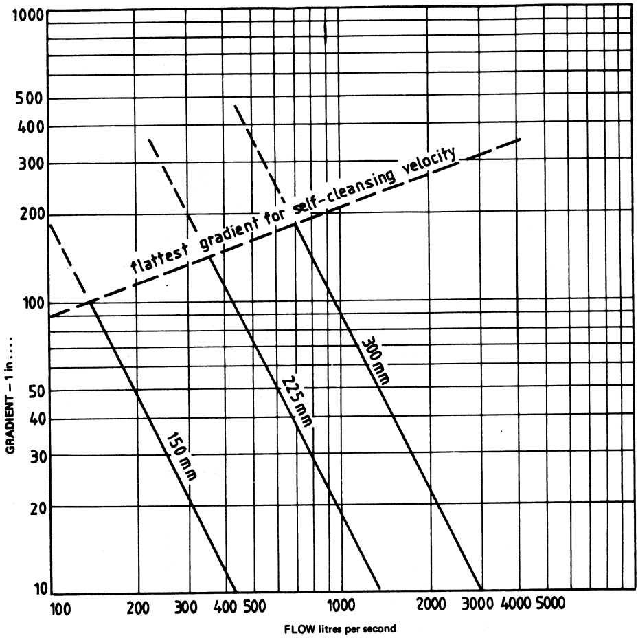
Fig. 7. FLOW IN SEWERS AND DRAINS
