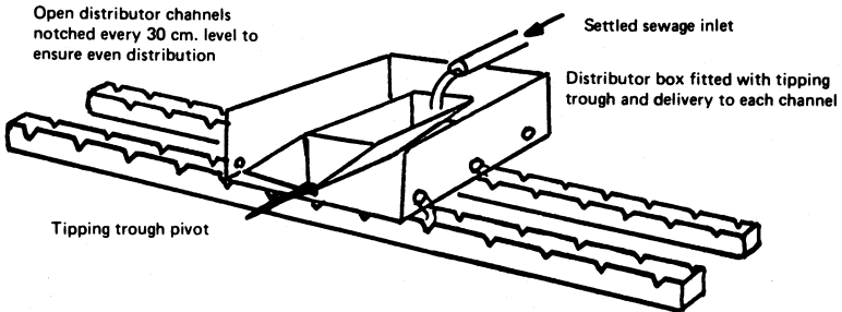
An alternative form of distributor for small filters
