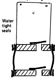
Section of bellows showing end discs, valves and top bracket
