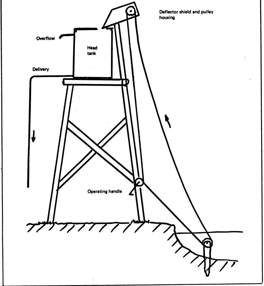
Fig. 16. THE ROPE LIFT
