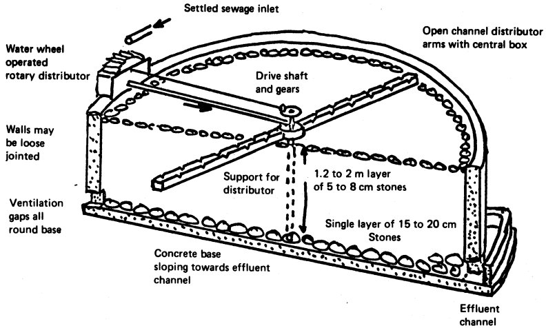
Fig. 32. PERCOLATING FILTERS
