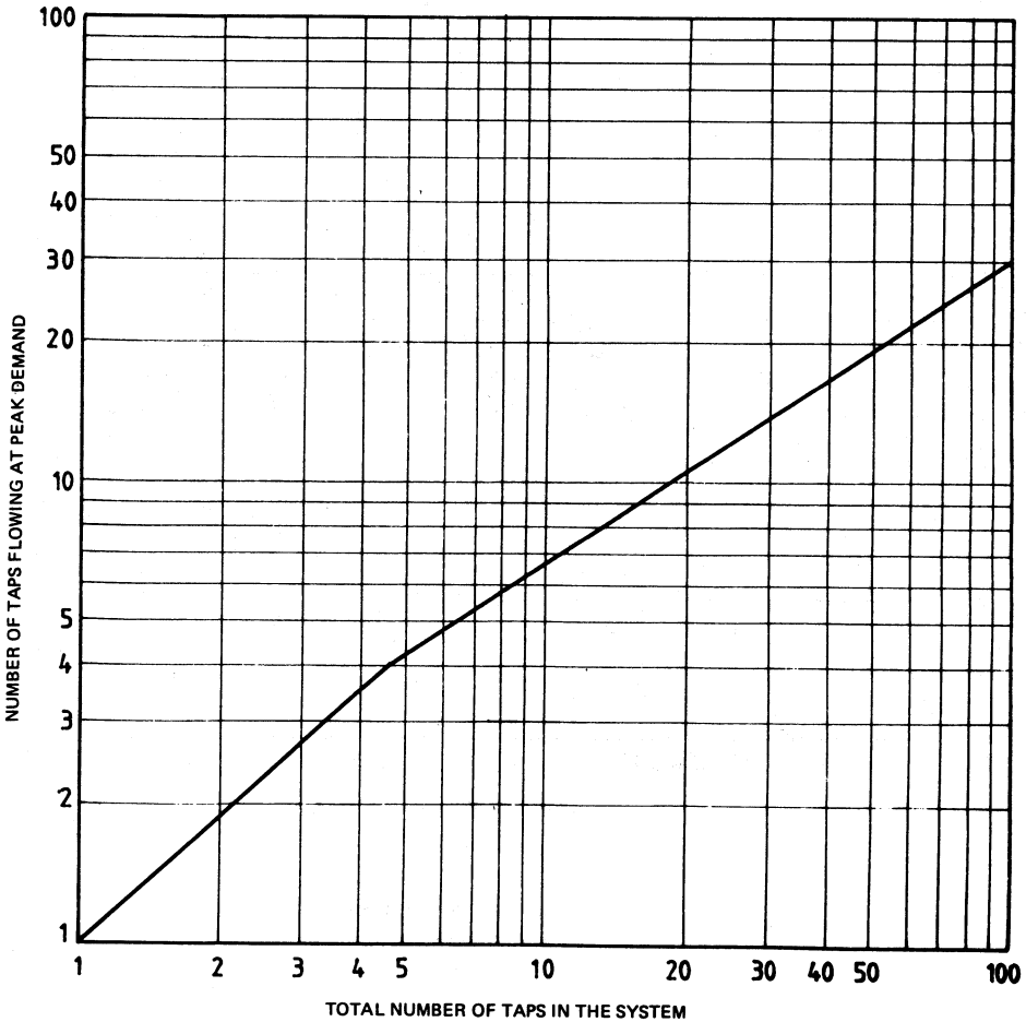
Fig. 6. INSTANTANEOUS DEMAND IN A SMALL WATER SYSTEM
