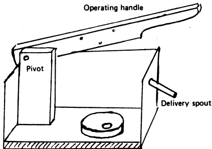
Assembly showing outer case made from debbi with reinforcement on bottomside
