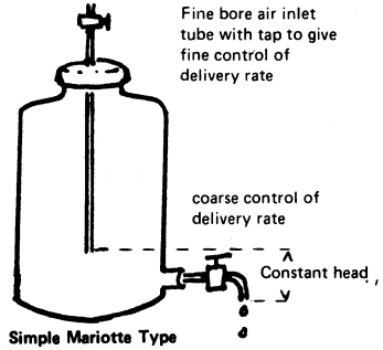
Fig. 20. DOSERS FOR CHEMICAL SOLUTIONS
