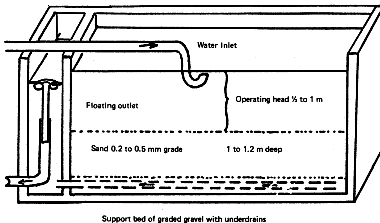
Fig. 22. SLOW SAND FILTER
