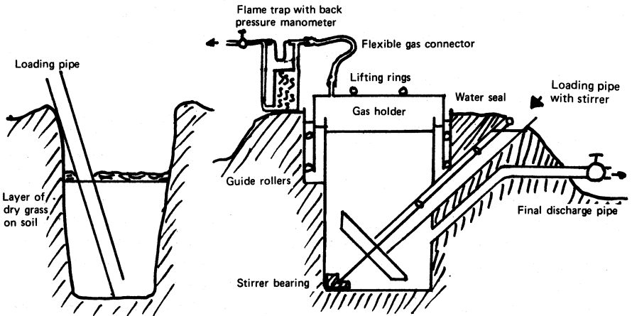
Fig. 36 ANAEROBIC SLUDGE DIGESTION FOR WARM CLIMATES
