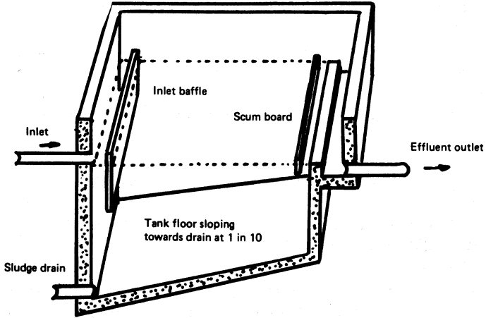
Horizontal flow type
