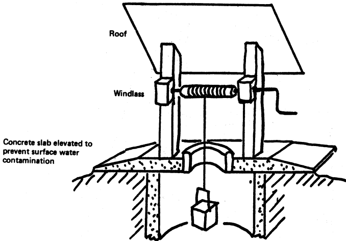
Fig. 17. BUCKET LIFTS IN SMALL WELLS
