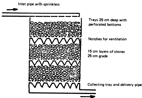
Fig. 25. TRICKLING FILTER FOR AERATION AND IRON REMOVAL
