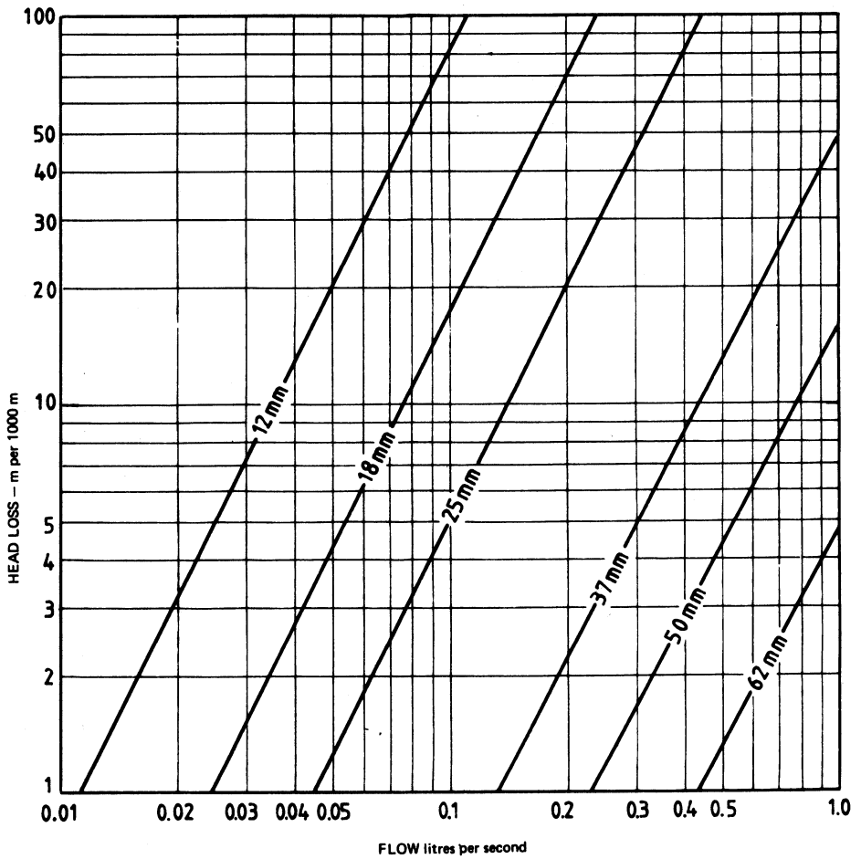
Fig. 5. HEAD LOSS IN PIPELINES (Galvanised Steel)
