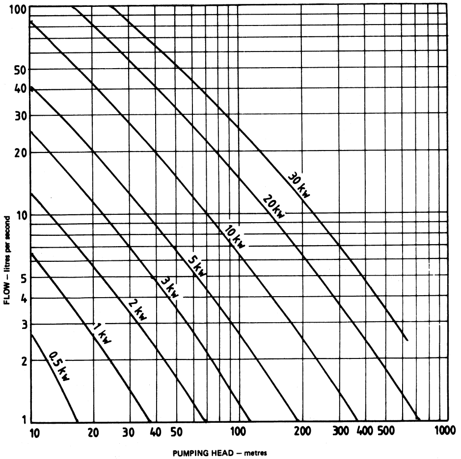
Fig. 11. KILOWATT DEMAND OF PUMPS REQUIRED TO PROVIDE VARIOUS FLOWS AT DIFFERENT PUMPING HEADS
