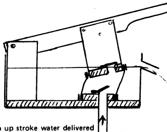
An improvised pump — using a bellows made from a short section cut from car inner tube and flap valves made from the same material
