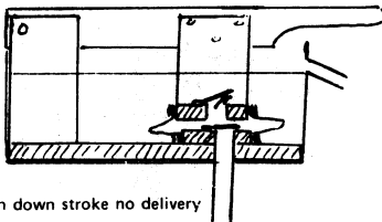
An improvised pump — using a bellows made from a short section cut from car inner tube and flap valves made from the same material
