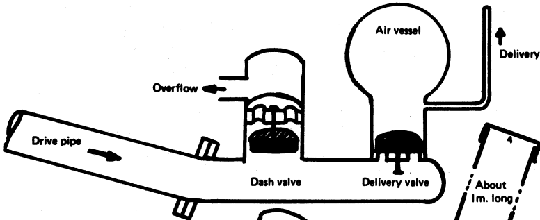
A Commercial Pump
