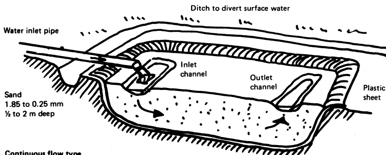
Fig. 24. THE HORIZONTAL SAND FILTER
