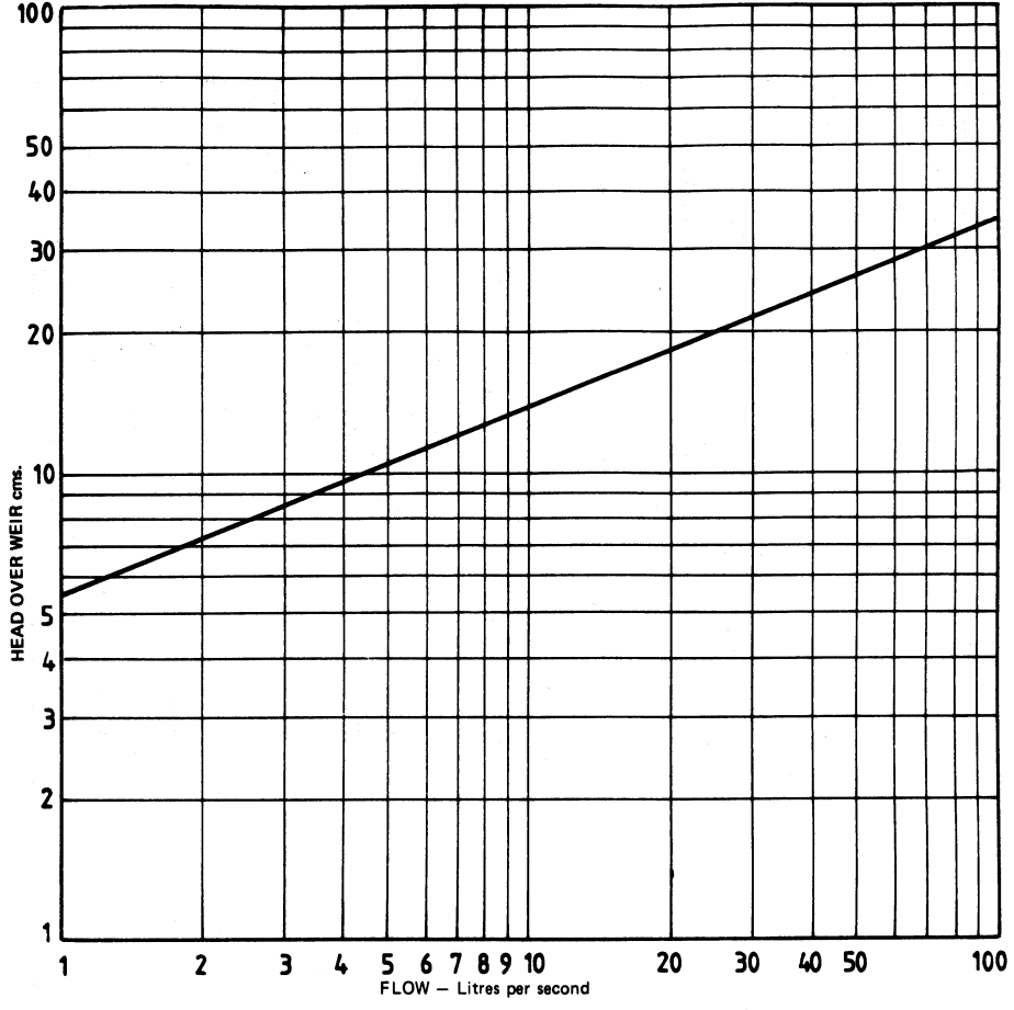
Fig. 9. FLOW MEASUREMENT WITH A 90° V-NOTCH WEIR
