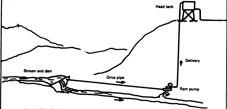
A typical Ram Pump installation
