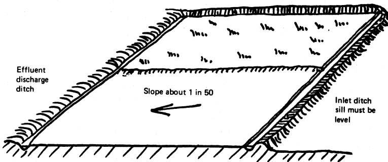
Fig. 35. GRASS PLOTS FOR FINAL EFFLUENT TREATMENT
