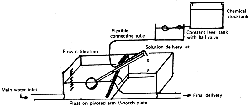
Variable head type coupled to V-notch measurement of flow gives a dose rate approximately proportional to flow
