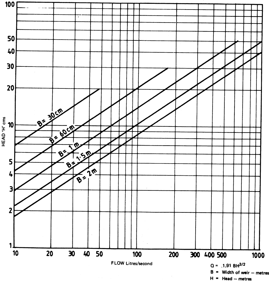
Fig. 10. MEASUREMENT OF FLOW OVER HORIZONTAL WEIRS
