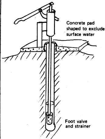
A typical installation
