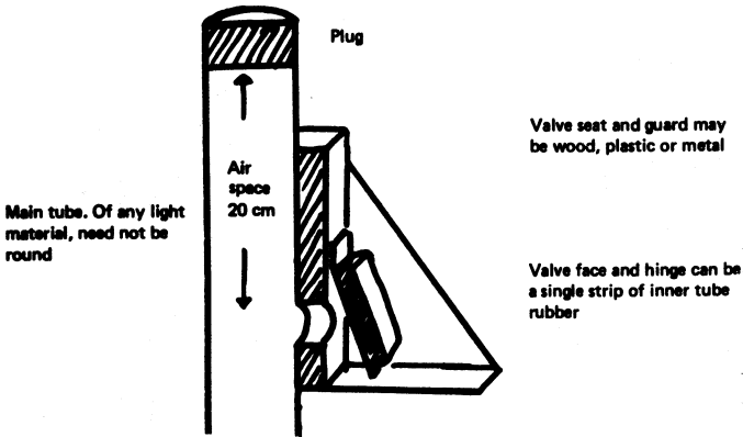
Fig. 15. THE SIMPLEST PUMP
