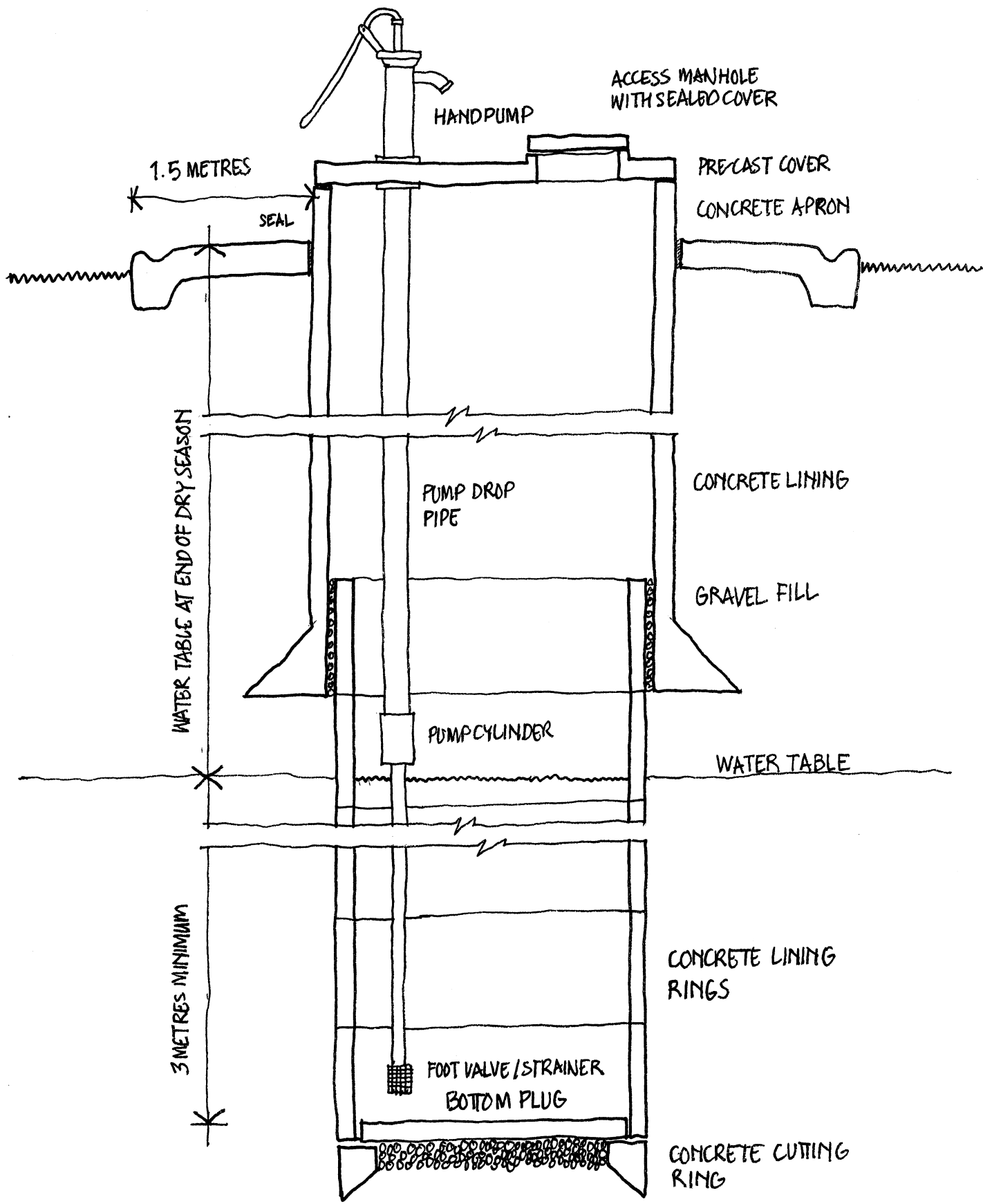
Figure 6: Details of typical concrete-lined and covered well
