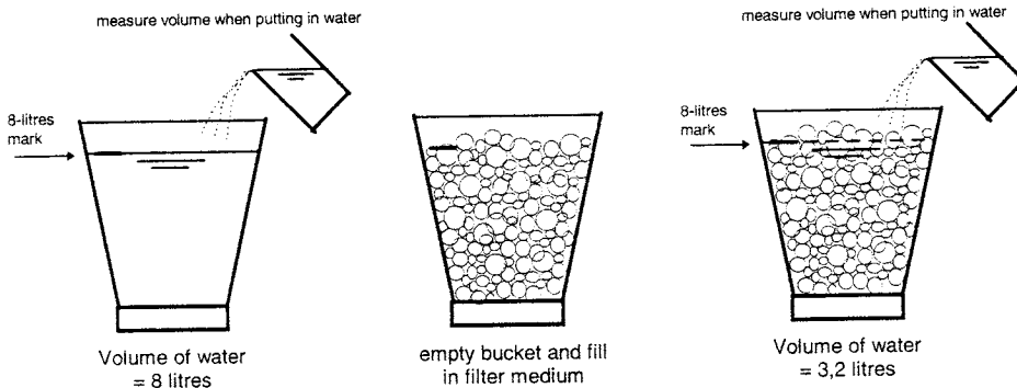
Fig. 35. Determining pore space of filter medium at site. For example the empty bucket is full after pouring 8 litre of water. The bucket filled with gravel absorbs 3.2 litre of water: Voids space is 3.2/8 = 0.40 or 40%.
