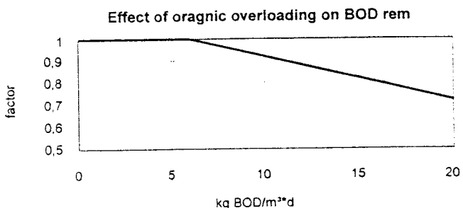
Fig. 77. BOD removal affected by organic overloading in baffled septic tanks
