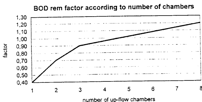
Fig. 78a. Influence of number of upflow chambers on BOD removal rate
