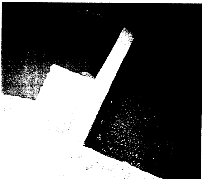
Fig. 9. Partition wall retaining scum. Inlet is at the right side, water flows below the partition wall into the compartment at the left side. [photo: Sasse]
