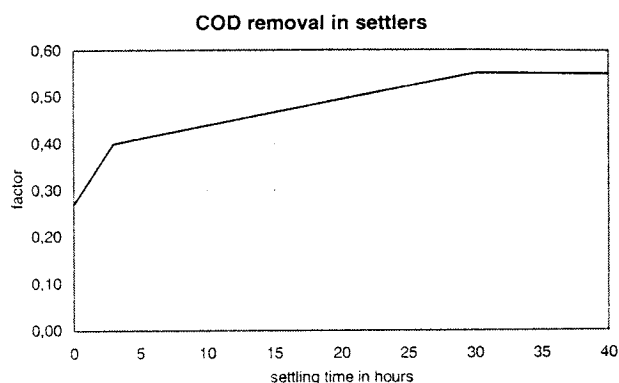
Fig. 68. COD removal in settlers
