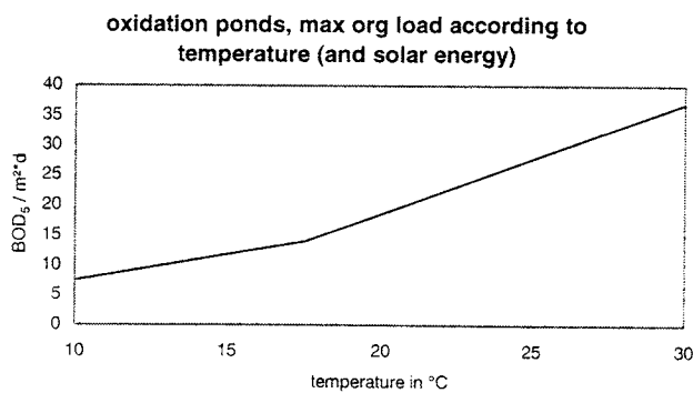
Fig. 89. Maximum organic load relative to temperature on aerobic-facultative oxidation ponds. The influence of sun-shine hours has been included.
