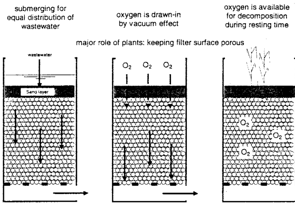
Fig. 32. The principle of the vertical filter
