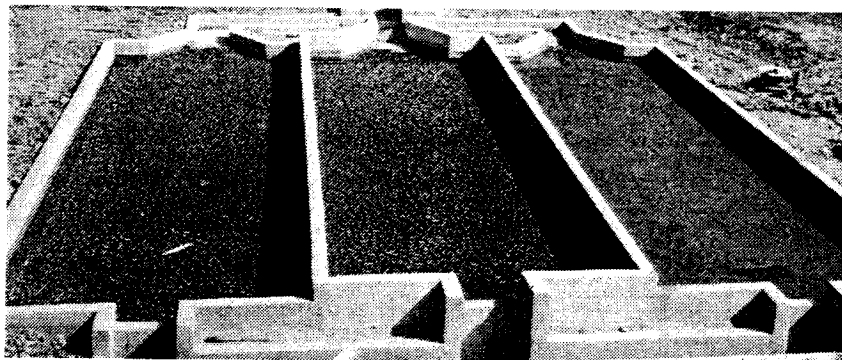
Fig. 55. Sludge drying beds constructed by University of Chiang Mei and GTZ in Thailand [photo: Sasse]
