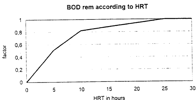
Fig. 76. BOD removal relative to HRT in baffled septic tanks
