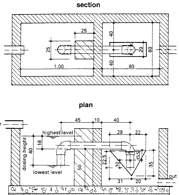
Fig. 39. Dosing chamber with tipping bucket for controlled operation of siphon. The bucket closes the siphon until it is filled with water. When losing its equilibrium due to the weight of the water, the bucket turns over and opens the siphon. It falls back into horizontal position to receive new water, which again closes the siphon for the next flush.
