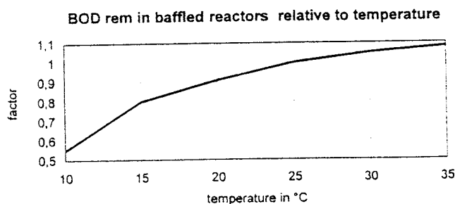
Fig. 78b. Influence of temperature on BOD removal rates in baffled septic tanks
