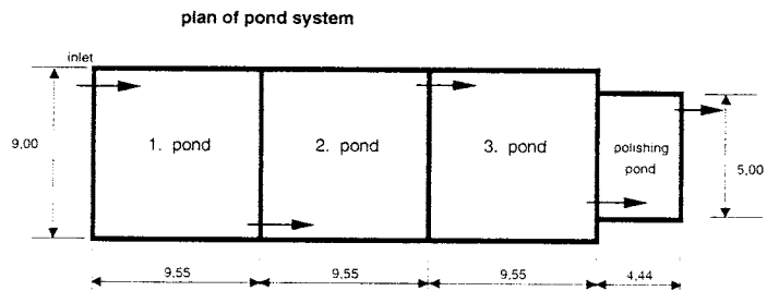
Fig. 92. Illustration to spread sheet for calculation of dimensions of aerobic-facultative ponds
