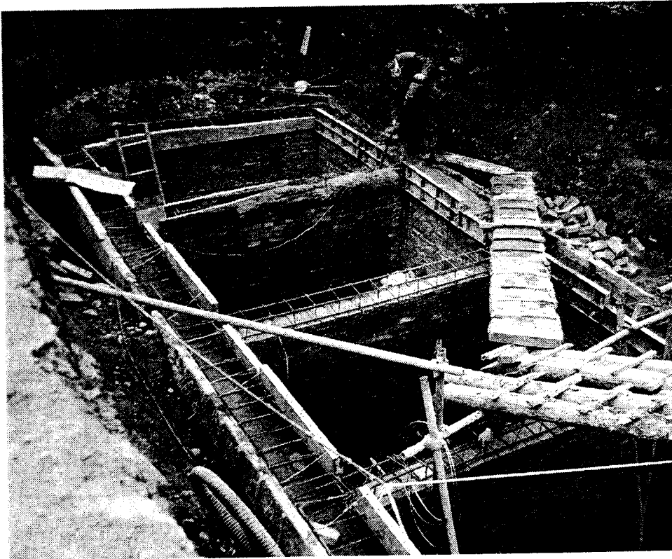
Fig. 3. DEWATS anaerobic filter under construction. Planning and supervision by CEEIC [photo: Sasse]
