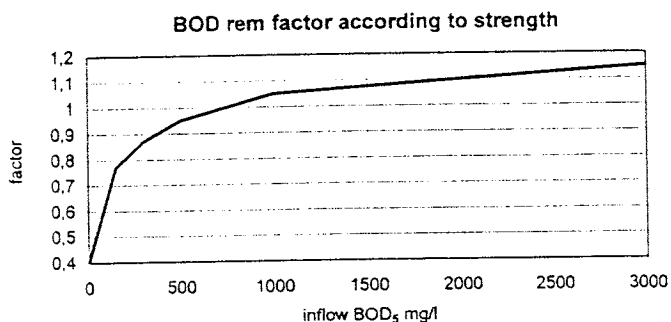
Fig. 78. BOD removal in baffled septic tanks related to wastewater strength
