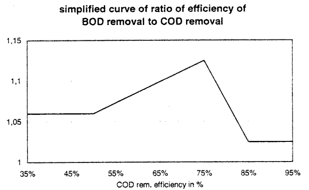
Fig. 65. Simplified curve of Fig. 64. which is used in the spread sheet formulas.
