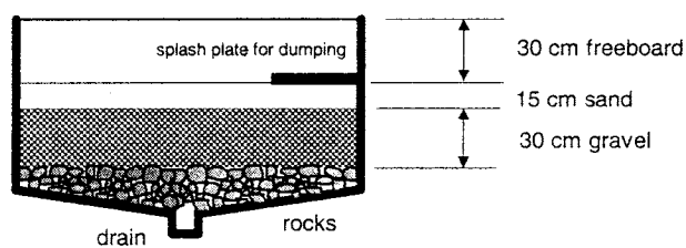
principle cross section of sludge drying bed
