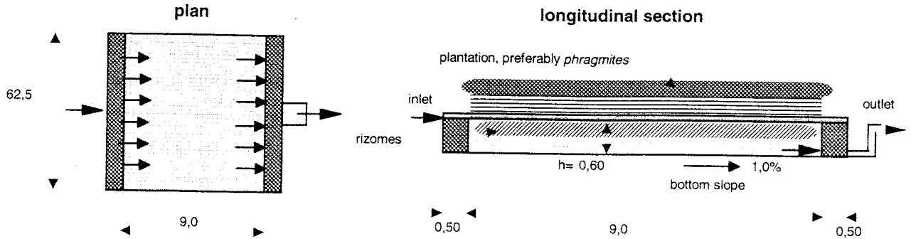
Fig. 85. Illustration to spread sheet for calculation of dimensions of horizontal gravel filters
