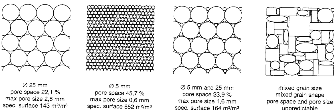
Fig. 33. Influence of grain size and shape on filter properties
