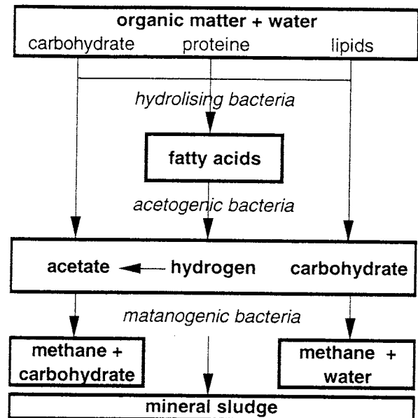
Fig. 7. The anaerobic process in principle
