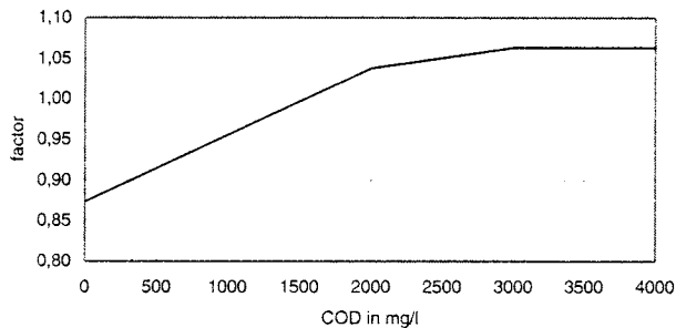
Fig. 73. COD removal relative to wastewater strength in anaerobic filters
