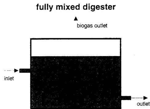
Fig. 28. Flow principle of the fully mixed anaerobic digester. There is only little sedimentation due to viscous substrate. All fractions of the substrate stay for the same period of time inside the digester. The position of inlet and outlet is less important with homogeneous liquid of high TS content. Small baffles may be provided to avoid short circuit of substrate.
