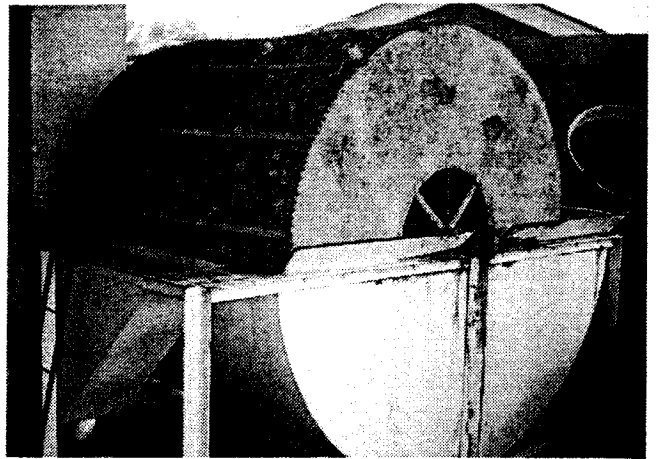
Fig. 52. Rotating disk reactor in a slaughter house in Jakarta, Indonesia. The reactor was temporarily out of use when the photograph was taken. [photo: Sasse]
