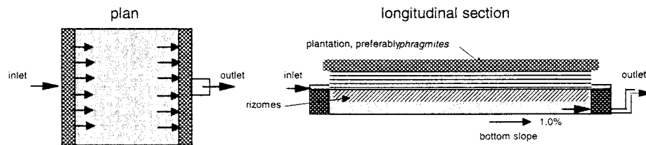
Fig. 31. The principle of the horizontal filter
