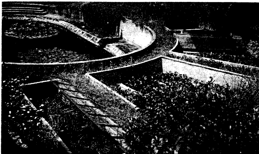
Fig. 48. Wastewater treatment tanks using aquatic plants in Auroville / India. The plant is placed directly beside residential houses. Lizards which live among the water hyacinth take care of mosquito control. The first settling tank is sealed against bad odour by a thick layer of scum on which papyrus grows (see Fig. 46). [photo: Sasse]
