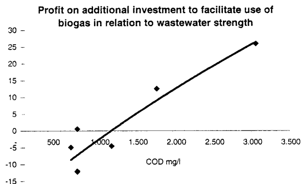
Fig. 5. Cost-benefit relation of biogas utilisation. It is not economical to use biogas from low strength wastewater.
