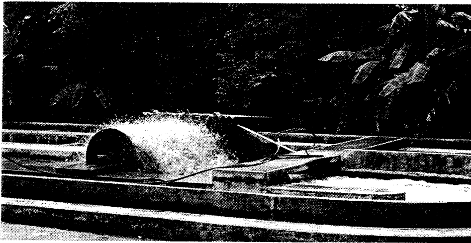
Fig. 53. Oxidation ditch operated at a rubber factory in Kerala / India [photo: Sasse]
