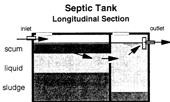
Fig. 17. Flow principle of the septic tank. Most sludge and scum is retained in the first chamber; the second chamber contains only little sludge which allows the water to flow undisturbed by rising gas bubbles.
