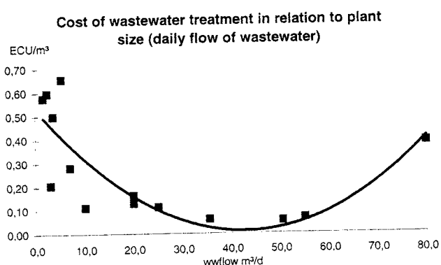
Fig. 4. Cost of treatment per m 3 daily flow. Larger plants require a more sophisticated technology which may increase treatment costs.
