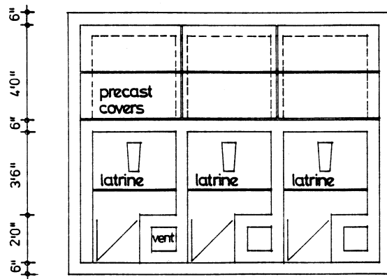
PIT LATRINE/3 FLOOR PLAN
