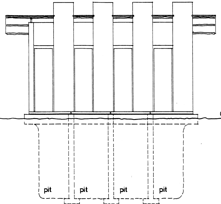
ENTRANCE ELEVATION
