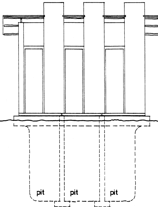
ENTRANCE ELEVATION
