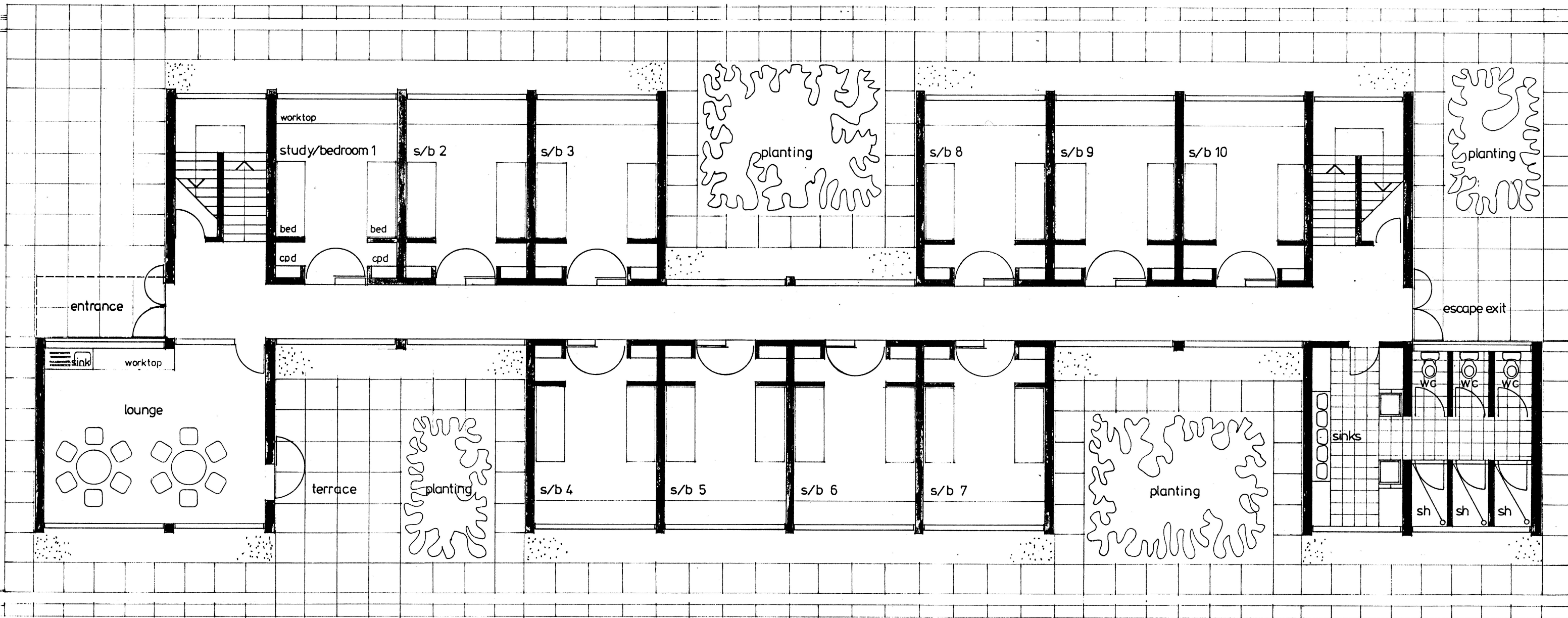
ground floor plan / 1/8" - 1'0"
