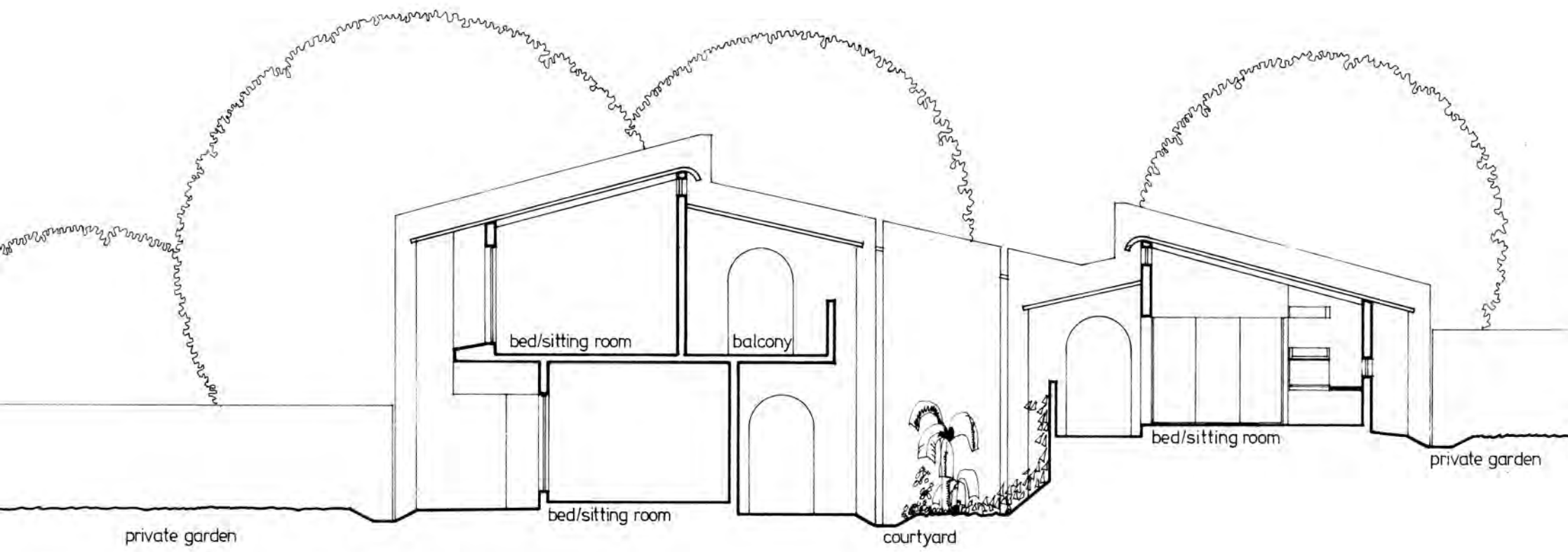
typical section
