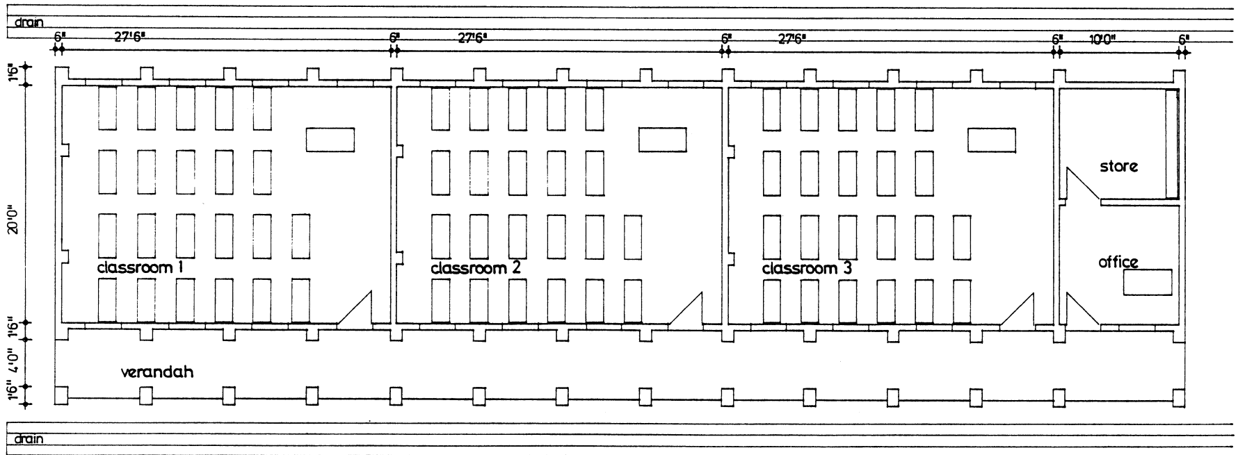
FLOOR PLAN PPS/5 : 3 CLASSROOM UNIT - PLAN & ELEVATIONS
