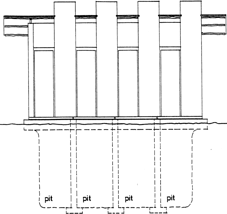
ENTRANCE ELEVATION
