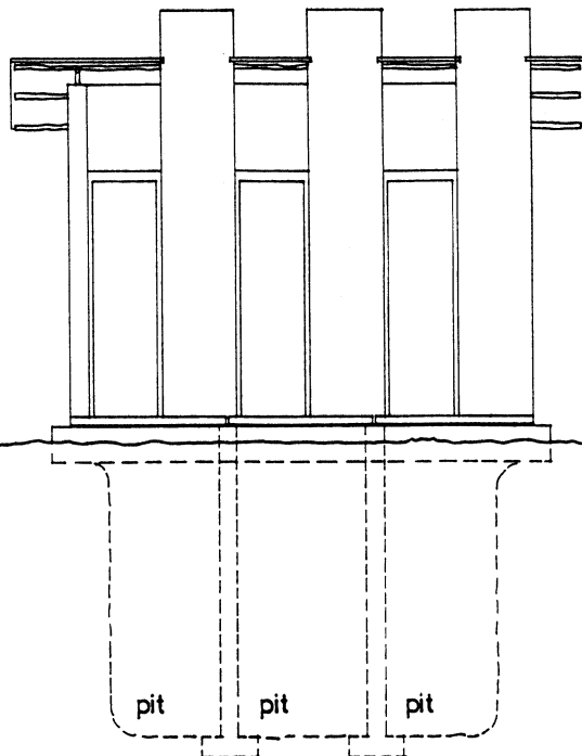
ENTRANCE ELEVATION
