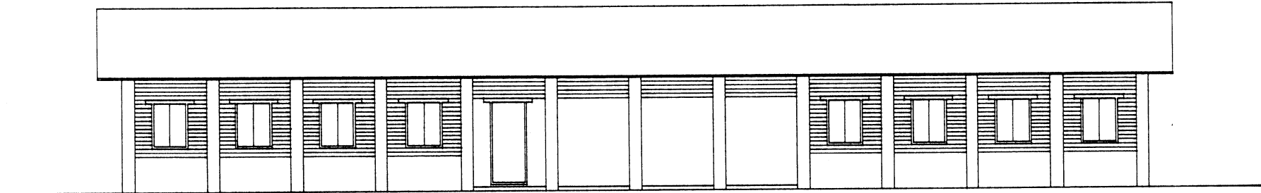
FRONT/ENTRANCE ELEVATION
