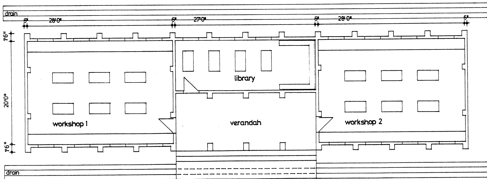
FLOOR PLAN
