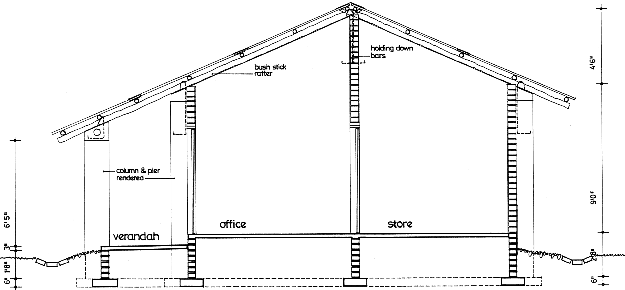
SECTION THRO' OFFICE & STORE
