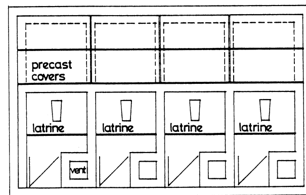
PIT LATRINE/4 FLOOR PLAN
