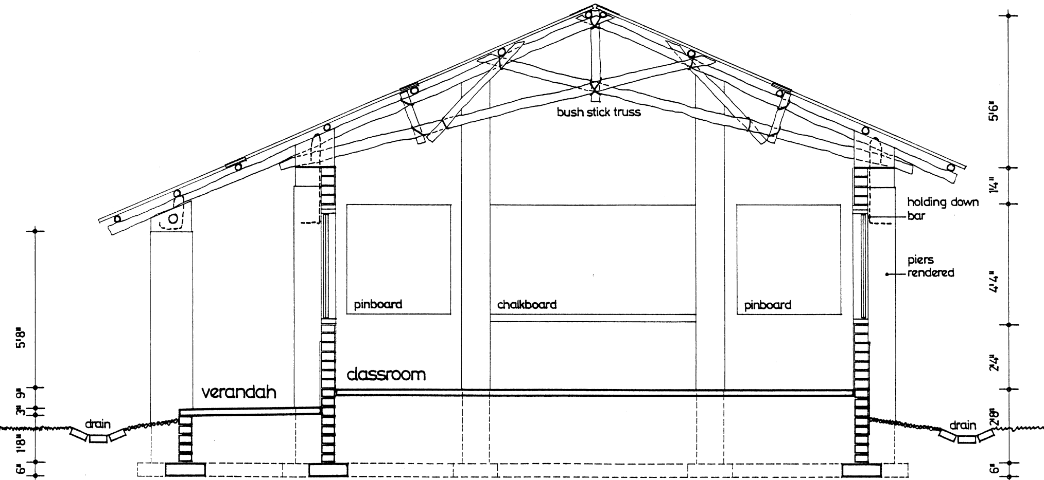
TYPICAL SECTION THRO' CLASSROOM
