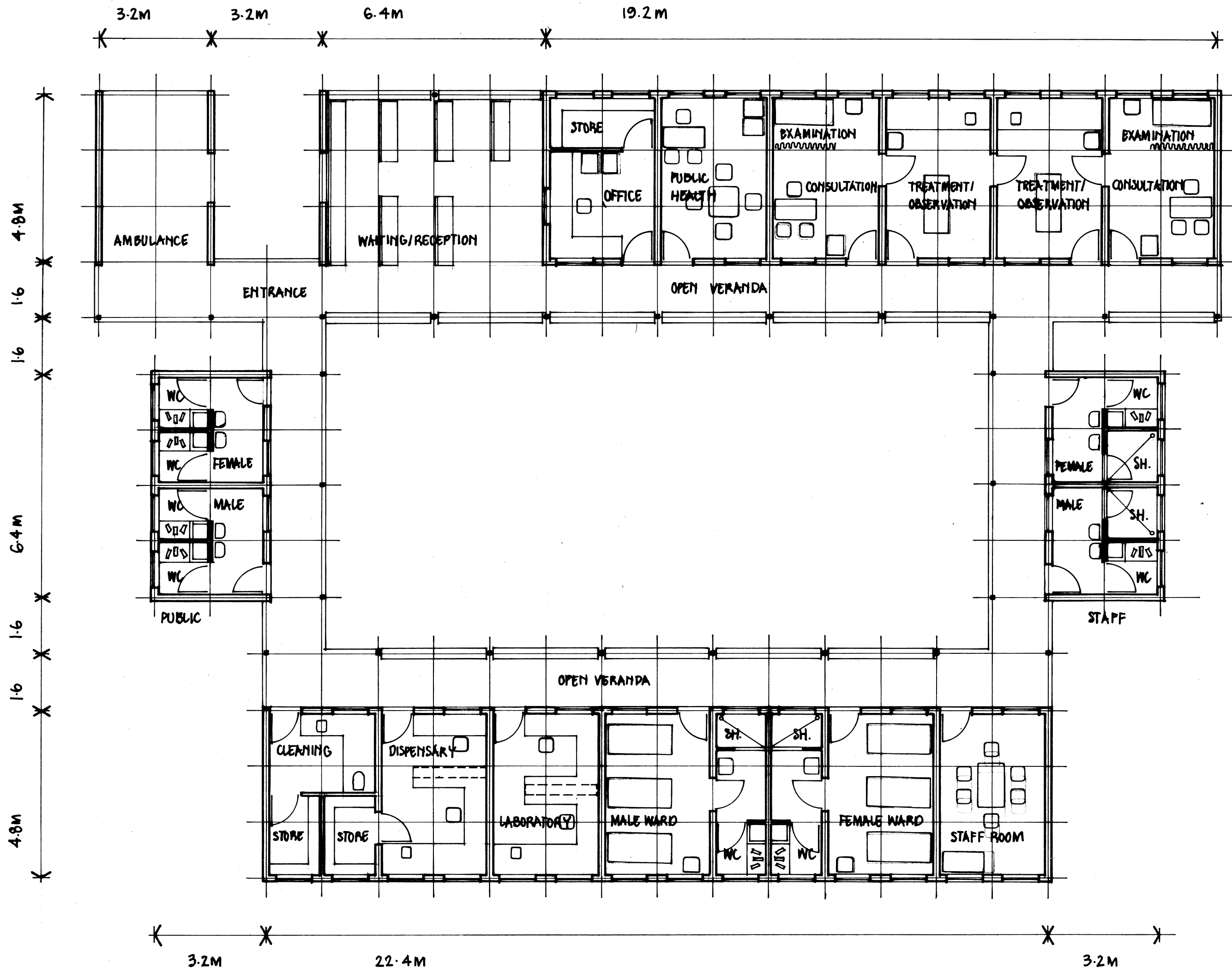
6-BED RURAL HOSPITAL - PRELIMINARY DESIGN
