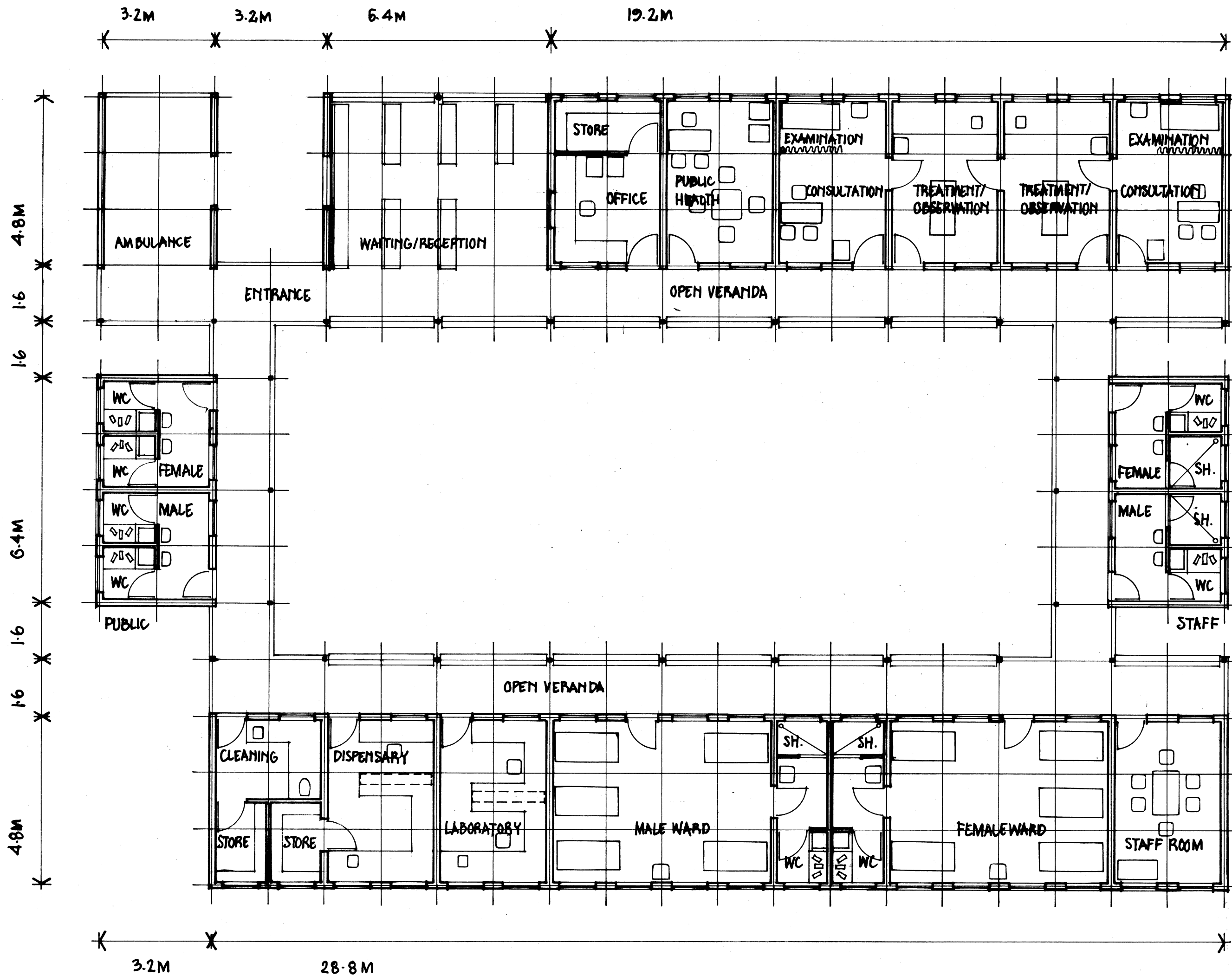
10-BED RURAL HOSPITAL - PRELIMINARY DESIGN
