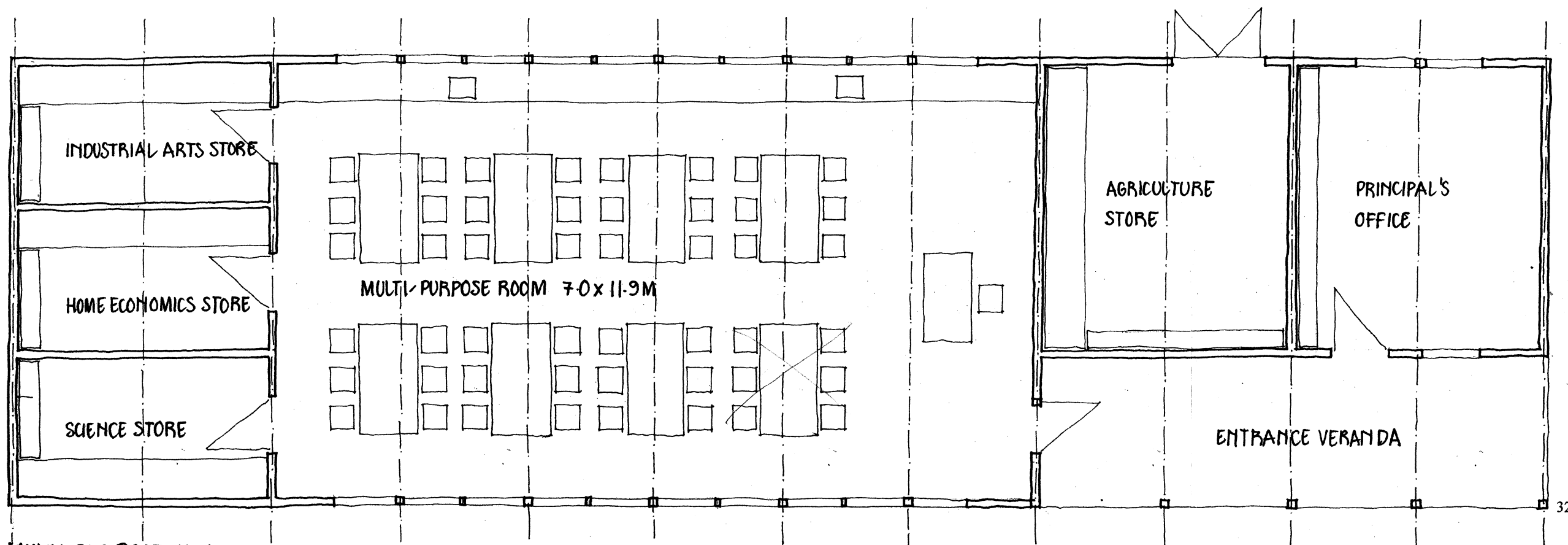
FIG.5 MULTI-PURPOSE UNIT
