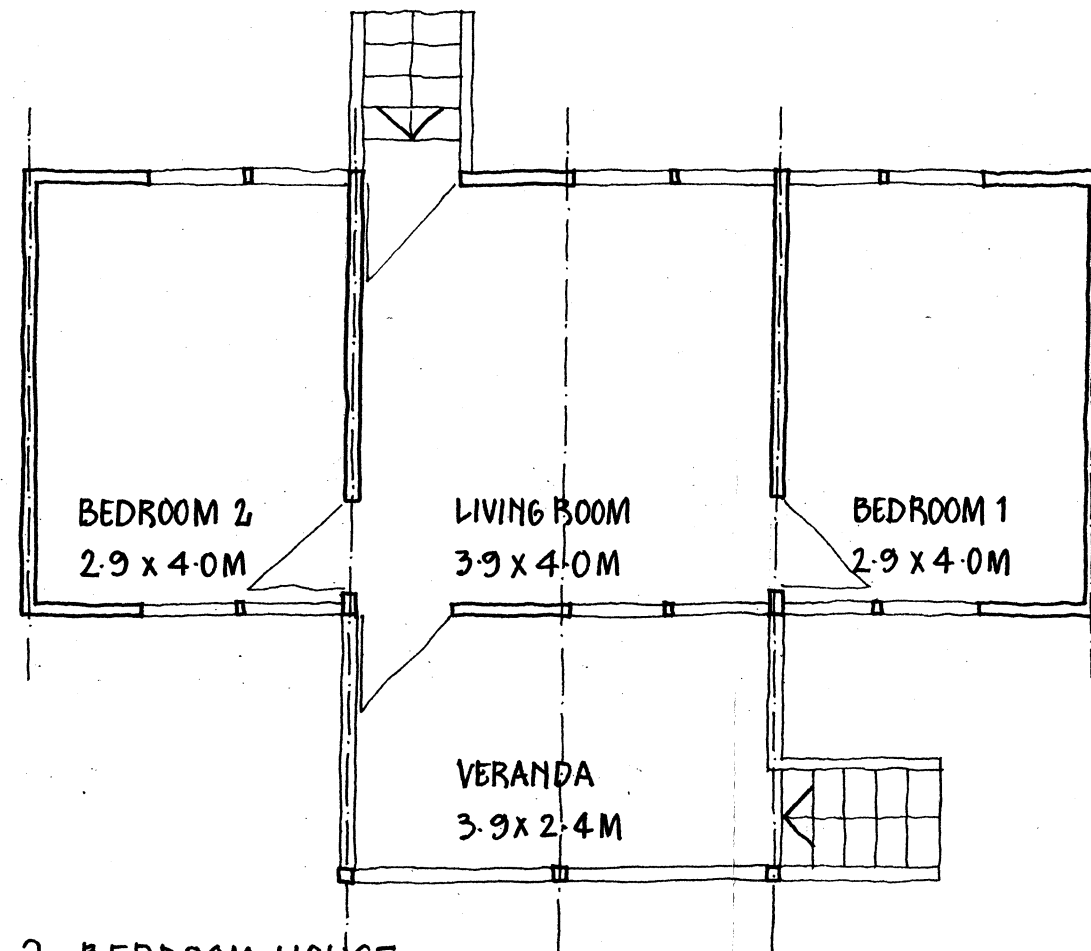
FIG. 8 2-BEDROOM HOUSE
