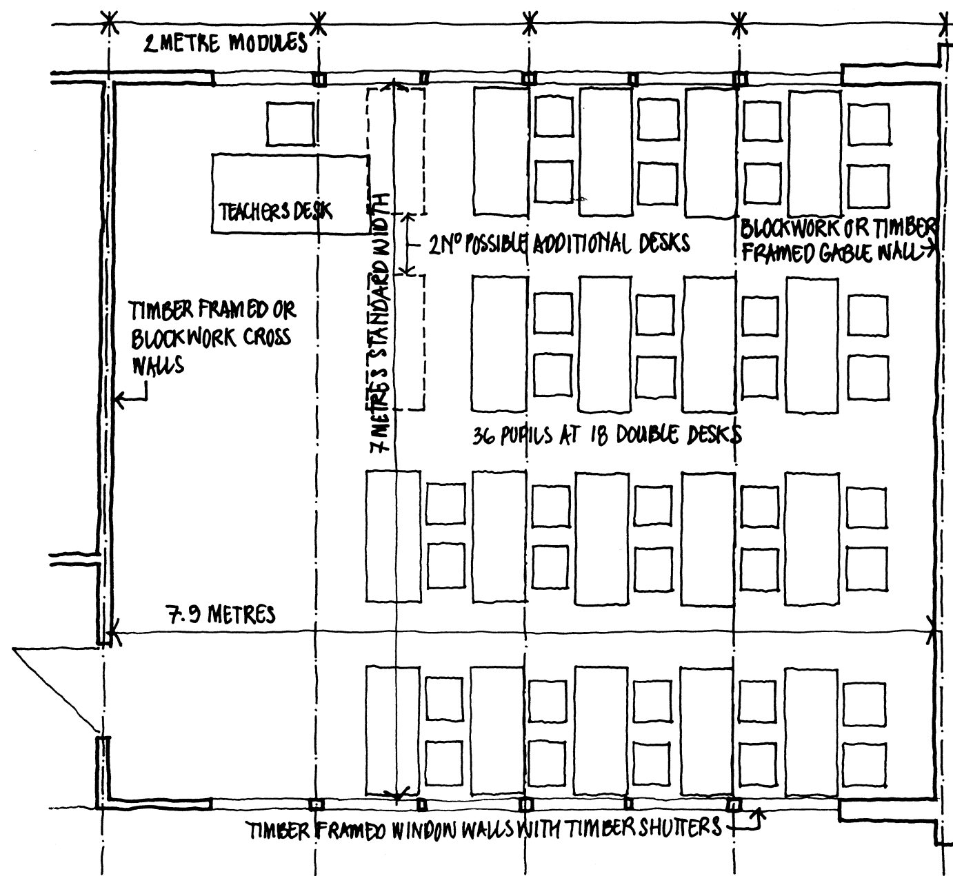
Figure 1: Standard Classroom layout showing 2-metre module, furniture layout and different construction materials.
