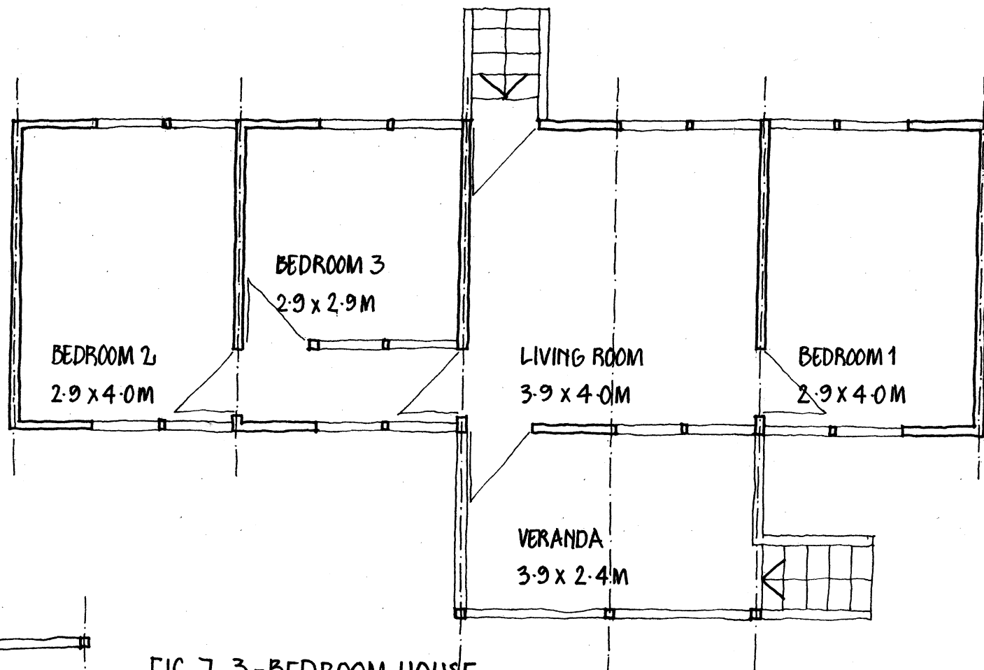
FIG. 7 3-BEDROOM HOUSE
