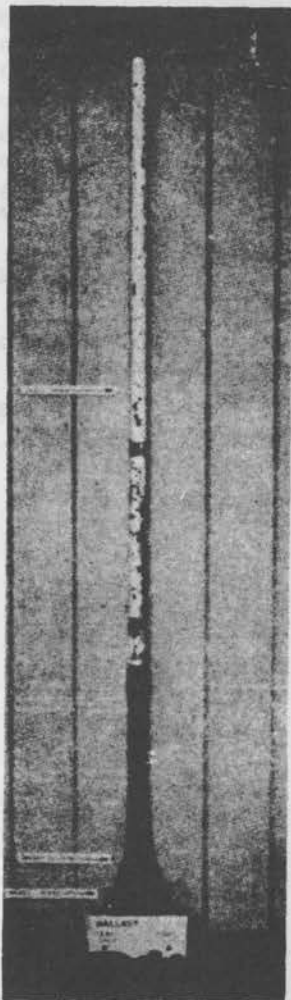
Figure 79a. Lift-drop tamper.
