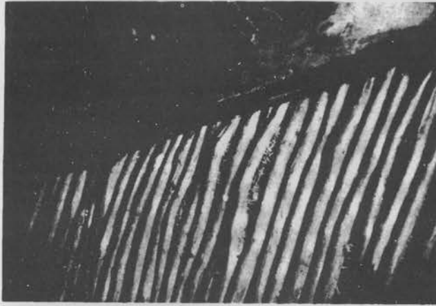
Figure 87. To compensate for the unevenness of the tops of the vigas, saplings can be placed diagonally for sheathing. Note the straw used in this case to prevent the earth fill from sifting through the ceiling.
