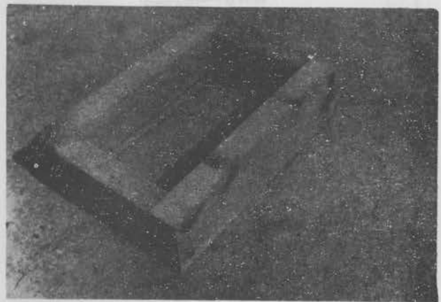
Figure 67a. This 2" x 4" wood nailer block, of the same dimensions as an adobe block, is inserted in place of the adobe block around windows and doors to offer an excellent, rigid hanger for the window or door frame.
