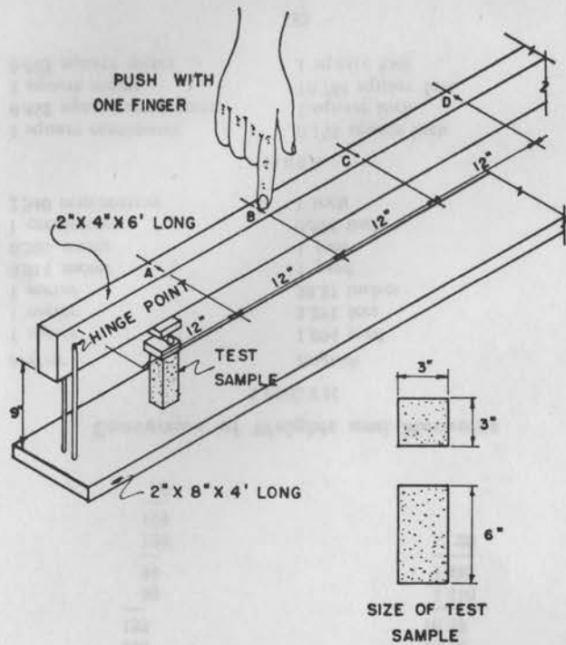
Figure 94. Simple lever tester for soils.
