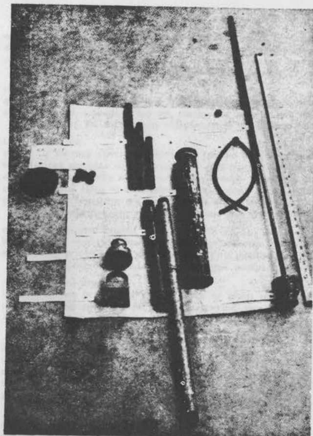
Figure 79c. Disassembled sliding weight tamper.
