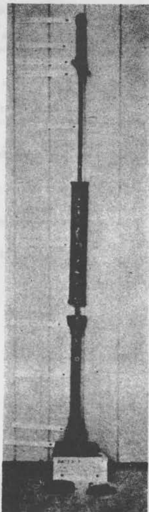
Figure 79b. Assembled sliding weight tamper.
