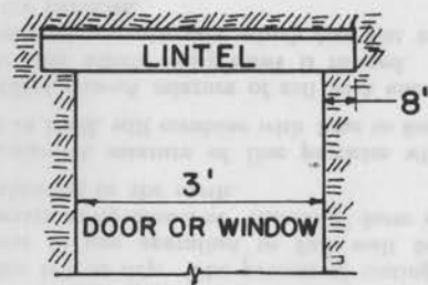
Figure 95. Wood lintel.
