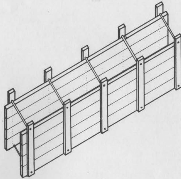
Figure 72. Form for ramming.
