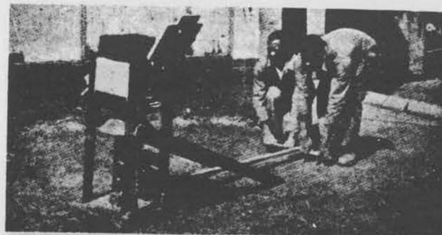
Figure 51. The compression and ejection stroke with this Ellson block-making machine consumed 1.4 seconds by stop watch.
