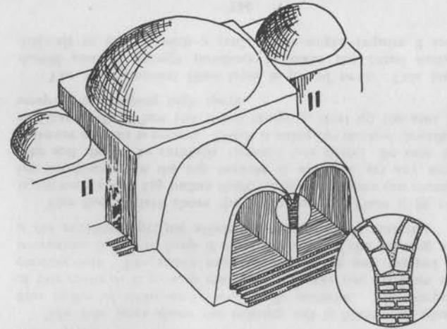
Figure 88. This style of earth dome and vault construction was used in a reconstruction program at New Gournia, Egypt.
