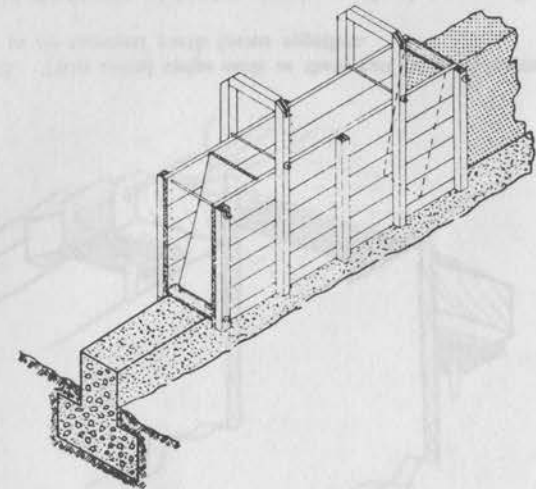
Figure 77. Form for ramming.
