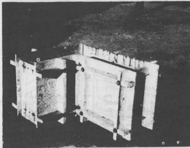
Figure 74. Plywood corner form for rammed earth walls.
