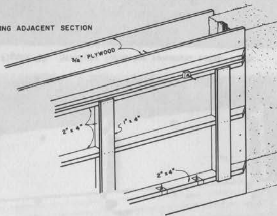
FORMING ADJACENT SECTION
