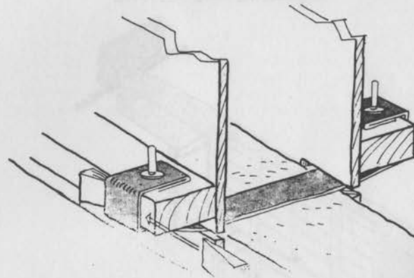
Figure 75. Thin metal strips such as these can be used instead of bolts to tie rammed earth forms together.
