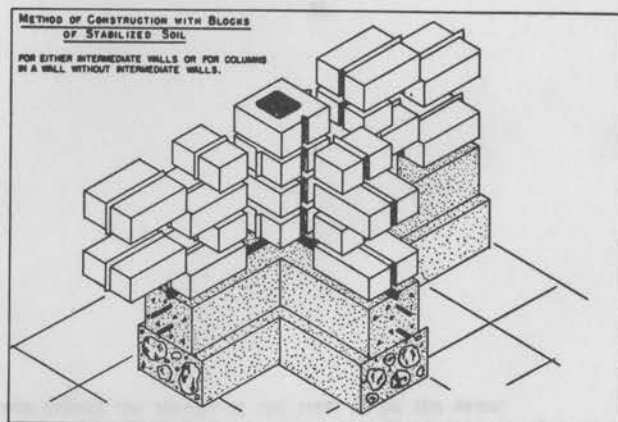
Figure 49. The various shapes of blocks produced by the Land-concrete block-making machine allow rigid construction of corners and tees.
