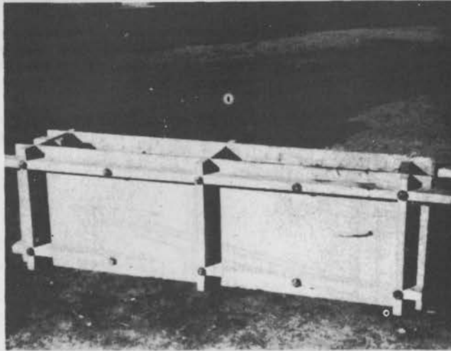
Figure 73. Straight form for rammed earth walls.
