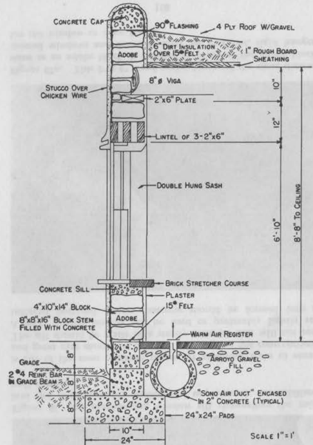
Figure 64. A builder in Albuquerque, N. M., uses this wall section for adobe walls.
